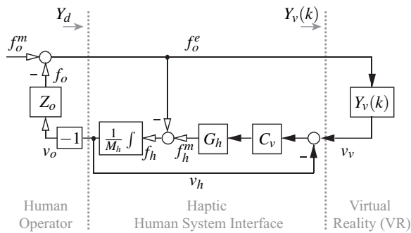
Figure 6: Admittance control: The haptic virtual reality is induced using different stiffnesses. High performance is achieved through light weighted robot.
