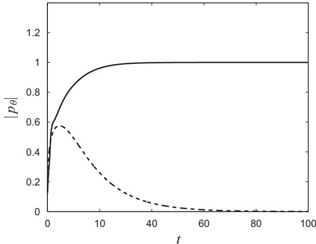
Fig. 2. Comparison of the behavior of the synchronization parameter |p_\theta| for two different local information algorithms when the initial conditions spread over the entire circle: the (dynamic) algorithm (15) (full line); the (static) algorithm (11) (dash line). Only the first algorithm achieves synchronization. The simulation involves N = 20 particles with a random initial condition.
