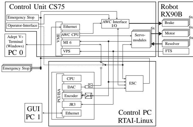
Fig. 1. Open control architecture with Stäubli RX90B and a control PC
