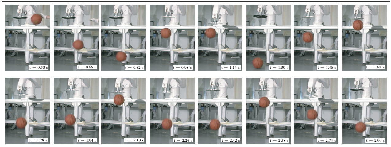
Fig. 6. Experimental snapshots of vision-based dribbling with initialization by human operator (sequence from 0.5 s to 2.9 s)
