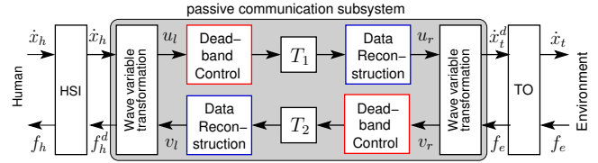
Figure 6: Deadband controlled haptic telepresence system.
