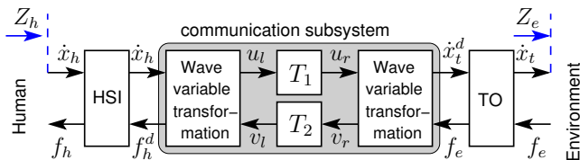
Figure 2: System architecture with wave variable transformation.
