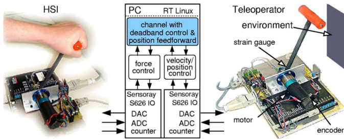
Fig. 6. Experimental setup with two 1-DoF haptic devices.
