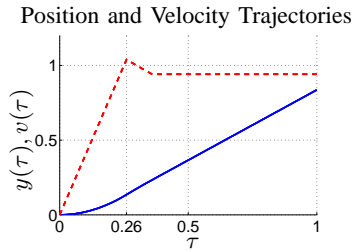
Fig. 2. Optimal position y(\tau) (blue, solid) and velocity v(\tau) (red, dashed) over time \tau .
