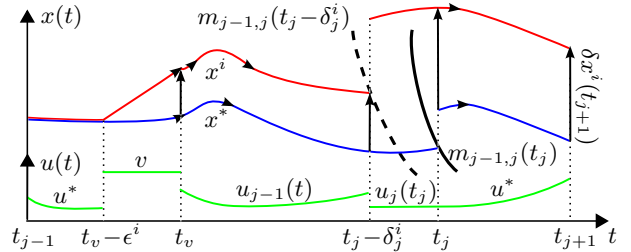
Fig. 1. Optimal and perturbed state trajectory with corresponding perturbed continuous control trajectory.
